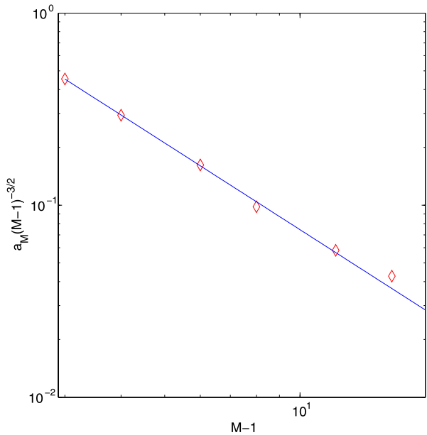
Fig. 6 The intercepts of Fig. 5 as a function of M - 1 at temperature T = 0.6 in log-log scale. The straight line is the best fit of the form a(M - 1)^{-3/2}
