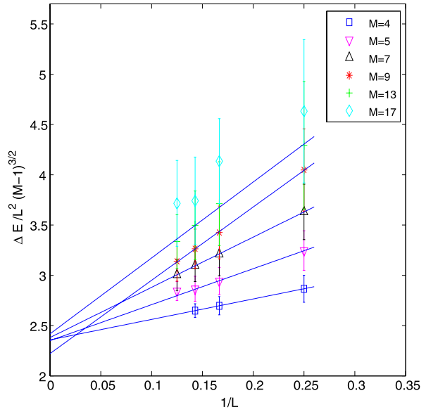
Fig. 5 \frac{\Delta E}{L^2}(M-1)^{3/2} versus 1/L at temperature T = 0.6
