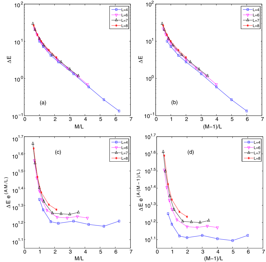
Fig. 3 \Delta E as a function of M/L (panel (a)) and as a function of (M - 1)/L (panel (b)) at temperature T = 1.1 ; \Delta E e^{AM/L} as a function of M/L (panel (c)) and \Delta E e^{A(M-1)/L} as a function of (M - 1)/L (panel (d)). A is 0.77. In each panel the different curves refer to different L values
