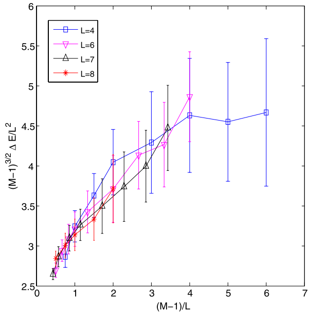
Fig. 7 \frac{\Delta E}{L^2}(M-1)^{3/2} versus (M-1)/L at temperature T = 0.6
